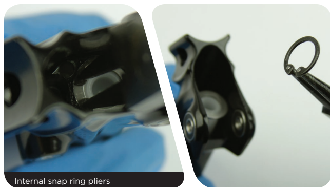
Internal snap ring pliers
